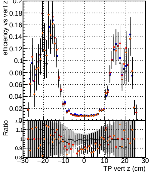
Efficiency vs vert z —•— DQM_mkFit_TTbase —•— DQM_mkFit5_TT_retrainOldFiles125_v2_prelimWP_epoch4 —•— DQM_mkFit_TT_baseline_6iter —•— DQM_mkFit6_TT_retrainOldFiles125_v2_prelimWP_epoch4
