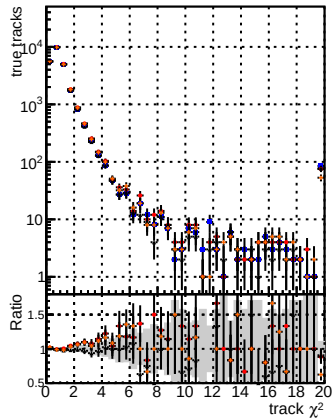
N of reco track vs. \chi^2 for BSM mFit 11, BSM mFit 12, BSM mFit 13, BSM mFit 14, BSM mFit 15, BSM mFit 16, BSM mFit 17, BSM mFit 18, BSM mFit 19, BSM mFit 20, BSM mFit 21, BSM mFit 22, BSM mFit 23, BSM mFit 24, BSM mFit 25, BSM mFit 26, BSM mFit 27, BSM mFit 28, BSM mFit 29, BSM mFit 30, BSM mFit 31, BSM mFit 32, BSM mFit 33, BSM mFit 34, BSM mFit 35, BSM mFit 36, BSM mFit 37, BSM mFit 38, BSM mFit 39, BSM mFit 40, BSM mFit 41, BSM mFit 42, BSM mFit 43, BSM mFit 44, BSM mFit 45, BSM mFit 46, BSM mFit 47, BSM mFit 48, BSM mFit 49, BSM mFit 50, BSM mFit 51, BSM mFit 52, BSM mFit 53, BSM mFit 54, BSM mFit 55, BSM mFit 56, BSM mFit 57, BSM mFit 58, BSM mFit 59, BSM mFit 60, BSM mFit 61, BSM mFit 62, BSM mFit 63, BSM mFit 64, BSM mFit 65, BSM mFit 66, BSM mFit 67, BSM mFit 68, BSM mFit 69, BSM mFit 70, BSM mFit 71, BSM mFit 72, BSM mFit 73, BSM mFit 74, BSM mFit 75, BSM mFit 76, BSM mFit 77, BSM mFit 78, BSM mFit 79, BSM mFit 80, BSM mFit 81, BSM mFit 82, BSM mFit 83, BSM mFit 84, BSM mFit 85, BSM mFit 86, BSM mFit 87, BSM mFit 88, BSM mFit 89, BSM mFit 90, BSM mFit 91, BSM mFit 92, BSM mFit 93, BSM mFit 94, BSM mFit 95, BSM mFit 96, BSM mFit 97, BSM mFit 98, BSM mFit 99, BSM mFit 100
