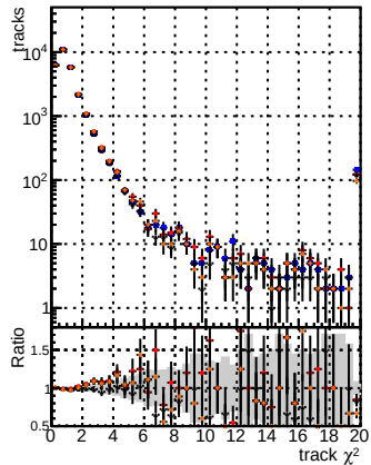
N of reco track vs. \chi^2 for BSM mFit 11, BSM mFit 12, BSM mFit 13, BSM mFit 14, BSM mFit 15, BSM mFit 16, BSM mFit 17, BSM mFit 18, BSM mFit 19, BSM mFit 20, BSM mFit 21, BSM mFit 22, BSM mFit 23, BSM mFit 24, BSM mFit 25, BSM mFit 26, BSM mFit 27, BSM mFit 28, BSM mFit 29, BSM mFit 30, BSM mFit 31, BSM mFit 32, BSM mFit 33, BSM mFit 34, BSM mFit 35, BSM mFit 36, BSM mFit 37, BSM mFit 38, BSM mFit 39, BSM mFit 40, BSM mFit 41, BSM mFit 42, BSM mFit 43, BSM mFit 44, BSM mFit 45, BSM mFit 46, BSM mFit 47, BSM mFit 48, BSM mFit 49, BSM mFit 50, BSM mFit 51, BSM mFit 52, BSM mFit 53, BSM mFit 54, BSM mFit 55, BSM mFit 56, BSM mFit 57, BSM mFit 58, BSM mFit 59, BSM mFit 60, BSM mFit 61, BSM mFit 62, BSM mFit 63, BSM mFit 64, BSM mFit 65, BSM mFit 66, BSM mFit 67, BSM mFit 68, BSM mFit 69, BSM mFit 70, BSM mFit 71, BSM mFit 72, BSM mFit 73, BSM mFit 74, BSM mFit 75, BSM mFit 76, BSM mFit 77, BSM mFit 78, BSM mFit 79, BSM mFit 80, BSM mFit 81, BSM mFit 82, BSM mFit 83, BSM mFit 84, BSM mFit 85, BSM mFit 86, BSM mFit 87, BSM mFit 88, BSM mFit 89, BSM mFit 90, BSM mFit 91, BSM mFit 92, BSM mFit 93, BSM mFit 94, BSM mFit 95, BSM mFit 96, BSM mFit 97, BSM mFit 98, BSM mFit 99, BSM mFit 100
