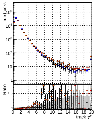
N of reco track vs. \chi^2 for BSM mFit, BSM mFit + base, BSM mFit + base + OldFiles125 v2_prelimWP_epoch4
