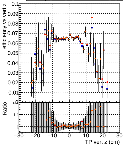
Efficiency vs vert z DOM_mkFit_TTbase DOM_mkFit5_TT_retrainOldFiles125_v2_prelimWP_epoch4 DOM_mkFit_TT_baseline_6iter DOM_mkFit6_TT_retrainOldFiles125_v2_prelimWP_epoch4
