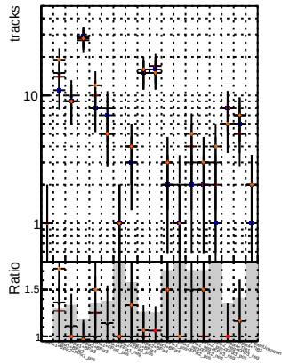
N of reco track vs. \chi^2 for BSM mFit TTbase, BSM mFit TTbase + 1-loop, BSM mFit TTbase + 1-loop + 2-loop, BSM mFit TTbase + 1-loop + 2-loop + 3-loop, BSM mFit TTbase + 1-loop + 2-loop + 3-loop + 4-loop, BSM mFit TTbase + 1-loop + 2-loop + 3-loop + 4-loop + 5-loop, BSM mFit TTbase + 1-loop + 2-loop + 3-loop + 4-loop + 5-loop + 6-loop, BSM mFit TTbase + 1-loop + 2-loop + 3-loop + 4-loop + 5-loop + 6-loop + 7-loop, BSM mFit TTbase + 1-loop + 2-loop + 3-loop + 4-loop + 5-loop + 6-loop + 7-loop + 8-loop, BSM mFit TTbase + 1-loop + 2-loop + 3-loop + 4-loop + 5-loop + 6-loop + 7-loop + 8-loop + 9-loop, BSM mFit TTbase + 1-loop + 2-loop + 3-loop + 4-loop + 5-loop + 6-loop + 7-loop + 8-loop + 9-loop + 10-loop, BSM mFit TTbase + 1-loop + 2-loop + 3-loop + 4-loop + 5-loop + 6-loop + 7-loop + 8-loop + 9-loop + 10-loop + 11-loop, BSM mFit TTbase + 1-loop + 2-loop + 3-loop + 4-loop + 5-loop + 6-loop + 7-loop + 8-loop + 9-loop + 10-loop + 11-loop + 12-loop, BSM mFit TTbase + 1-loop + 2-loop + 3-loop + 4-loop + 5-loop + 6-loop + 7-loop + 8-loop + 9-loop + 10-loop + 11-loop + 12-loop + 13-loop, BSM mFit TTbase + 1-loop + 2-loop + 3-loop + 4-loop + 5-loop + 6-loop + 7-loop + 8-loop + 9-loop + 10-loop + 11-loop + 12-loop + 13-loop + 14-loop, BSM mFit TTbase + 1-loop + 2-loop + 3-loop + 4-loop + 5-loop + 6-loop + 7-loop + 8-loop + 9-loop + 10-loop + 11-loop + 12-loop + 13-loop + 14-loop + 15-loop, BSM mFit TTbase + 1-loop + 2-loop + 3-loop + 4-loop + 5-loop + 6-loop + 7-loop + 8-loop + 9-loop + 10-loop + 11-loop + 12-loop + 13-loop + 14-loop + 15-loop + 16-loop, BSM mFit TTbase + 1-loop + 2-loop + 3-loop + 4-loop + 5-loop + 6-loop + 7-loop + 8-loop + 9-loop + 10-loop + 11-loop + 12-loop + 13-loop + 14-loop + 15-loop + 16-loop + 17-loop, BSM mFit TTbase + 1-loop + 2-loop + 3-loop + 4-loop + 5-loop + 6-loop + 7-loop + 8-loop + 9-loop + 10-loop + 11-loop + 12-loop + 13-loop + 14-loop + 15-loop + 16-loop + 17-loop + 18-loop, BSM mFit TTbase + 1-loop + 2-loop + 3-loop + 4-loop + 5-loop + 6-loop + 7-loop + 8-loop + 9-loop + 10-loop + 11-loop + 12-loop + 13-loop + 14-loop + 15-loop + 16-loop + 17-loop + 18-loop + 19-loop, BSM mFit TTbase + 1-loop + 2-loop + 3-loop + 4-loop + 5-loop + 6-loop + 7-loop + 8-loop + 9-loop + 10-loop + 11-loop + 12-loop + 13-loop + 14-loop + 15-loop + 16-loop + 17-loop + 18-loop + 19-loop + 20-loop
