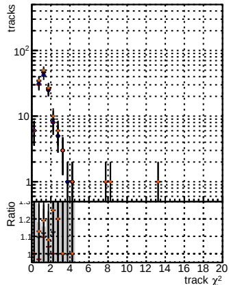
N of reco track vs. \chi^2 for BSM mFit TTbase, BSM mFit TTbase + 1-loop, BSM mFit TTbase + 1-loop + 2-loop, BSM mFit TTbase + 1-loop + 2-loop + 3-loop, BSM mFit TTbase + 1-loop + 2-loop + 3-loop + 4-loop, BSM mFit TTbase + 1-loop + 2-loop + 3-loop + 4-loop + 5-loop, BSM mFit TTbase + 1-loop + 2-loop + 3-loop + 4-loop + 5-loop + 6-loop, BSM mFit TTbase + 1-loop + 2-loop + 3-loop + 4-loop + 5-loop + 6-loop + 7-loop, BSM mFit TTbase + 1-loop + 2-loop + 3-loop + 4-loop + 5-loop + 6-loop + 7-loop + 8-loop, BSM mFit TTbase + 1-loop + 2-loop + 3-loop + 4-loop + 5-loop + 6-loop + 7-loop + 8-loop + 9-loop, BSM mFit TTbase + 1-loop + 2-loop + 3-loop + 4-loop + 5-loop + 6-loop + 7-loop + 8-loop + 9-loop + 10-loop, BSM mFit TTbase + 1-loop + 2-loop + 3-loop + 4-loop + 5-loop + 6-loop + 7-loop + 8-loop + 9-loop + 10-loop + 11-loop, BSM mFit TTbase + 1-loop + 2-loop + 3-loop + 4-loop + 5-loop + 6-loop + 7-loop + 8-loop + 9-loop + 10-loop + 11-loop + 12-loop, BSM mFit TTbase + 1-loop + 2-loop + 3-loop + 4-loop + 5-loop + 6-loop + 7-loop + 8-loop + 9-loop + 10-loop + 11-loop + 12-loop + 13-loop, BSM mFit TTbase + 1-loop + 2-loop + 3-loop + 4-loop + 5-loop + 6-loop + 7-loop + 8-loop + 9-loop + 10-loop + 11-loop + 12-loop + 13-loop + 14-loop, BSM mFit TTbase + 1-loop + 2-loop + 3-loop + 4-loop + 5-loop + 6-loop + 7-loop + 8-loop + 9-loop + 10-loop + 11-loop + 12-loop + 13-loop + 14-loop + 15-loop, BSM mFit TTbase + 1-loop + 2-loop + 3-loop + 4-loop + 5-loop + 6-loop + 7-loop + 8-loop + 9-loop + 10-loop + 11-loop + 12-loop + 13-loop + 14-loop + 15-loop + 16-loop, BSM mFit TTbase + 1-loop + 2-loop + 3-loop + 4-loop + 5-loop + 6-loop + 7-loop + 8-loop + 9-loop + 10-loop + 11-loop + 12-loop + 13-loop + 14-loop + 15-loop + 16-loop + 17-loop, BSM mFit TTbase + 1-loop + 2-loop + 3-loop + 4-loop + 5-loop + 6-loop + 7-loop + 8-loop + 9-loop + 10-loop + 11-loop + 12-loop + 13-loop + 14-loop + 15-loop + 16-loop + 17-loop + 18-loop, BSM mFit TTbase + 1-loop + 2-loop + 3-loop + 4-loop + 5-loop + 6-loop + 7-loop + 8-loop + 9-loop + 10-loop + 11-loop + 12-loop + 13-loop + 14-loop + 15-loop + 16-loop + 17-loop + 18-loop + 19-loop, BSM mFit TTbase + 1-loop + 2-loop + 3-loop + 4-loop + 5-loop + 6-loop + 7-loop + 8-loop + 9-loop + 10-loop + 11-loop + 12-loop + 13-loop + 14-loop + 15-loop + 16-loop + 17-loop + 18-loop + 19-loop + 20-loop
