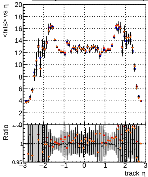
mean hits vs \eta DOM_mkFit_TTbase DOM_mkFit5_TT_retrainOldFiles125_v2_prelimWP_epoch4 DOM_mkFit_TT_baseline_6iter DOM_mkFit6_TT_retrainOldFiles125_v2_prelimWP_epoch4
