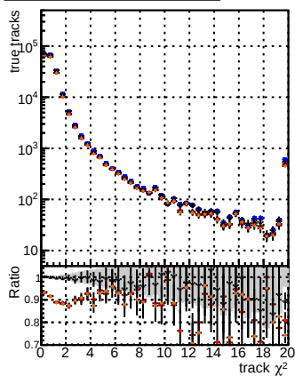
N of reco track vs. \chi^2 for BGM mkt15 (blue) and BGM mkt16 (orange) using the trainOldFiles125 v2_prelimWP_epoch4 and trainOldFiles125 v2_prelimWP_epoch4
