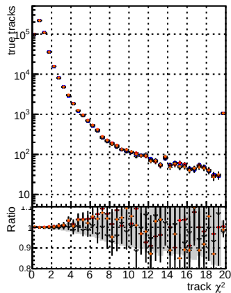
N of reco track vs. \chi^2 for BSM mFit v2 preliminary, TTbase, and BSM mFit v2 preliminary
