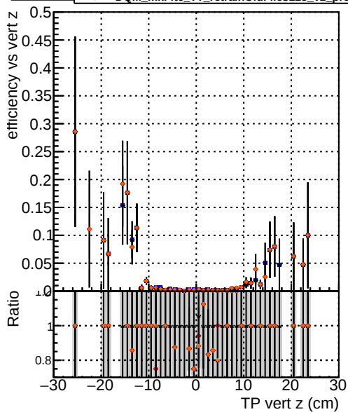
Efficiency vs vert z DOM_mkFit1_TTbase DOM_mkFit5_TT_retrainOldFiles125_v2_prelimWP_epoch4 DOM_mkFit6_TT_retrainOldFiles125_v2_prelimWP_epoch4 DOM_mkFit6_TT_baseline_6iter
