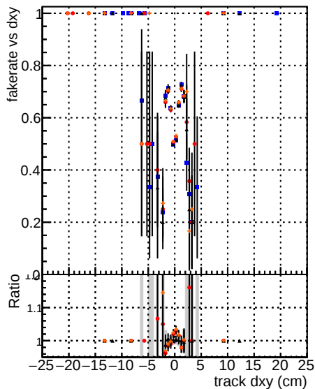
Legend: - \text{DGM\_mkFit\_TTbase} (blue circles) - \text{DGM\_mkFit\_TTbase\_trainOldFiles125\_v2\_prelimWP\_epoch4} (orange circles) - \text{DGM\_mkFit\_TTbase\_trainOldFiles125\_v2\_prelimWP\_epoch4} (red circles) - \text{DGM\_mkFit\_TTbase\_trainOldFiles125\_v2\_prelimWP\_epoch4} (black circles)
