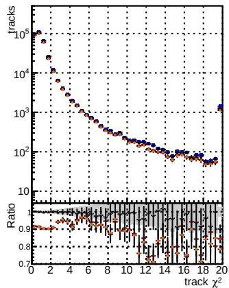
N of reco track vs. \chi^2 for BSM mFit TTbase, BSM mFit TTbase + trainOldFiles125 v2_prelimWP_epoch4, BSM mFit TTbase + trainOldFiles125 v2_prelimWP_epoch4
