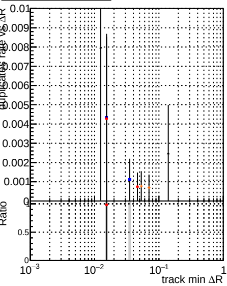
DOM mkFit TTbase DOM mkFit5 TTbase DOM mkFit6 TTbase DOM mkFit5 TT retrainOldFiles125_v2_prelimWP_epoch4
