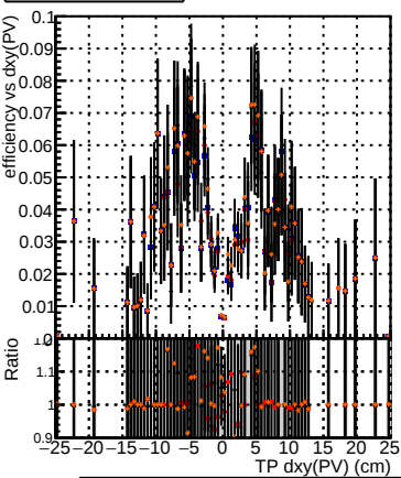
Efficiency vs Dxy(PV) Legend: DQM_mkFit5_QCDHighPt_base DQM_mkFit6_QCDHighPt_retrainOldFiles125_v2_prelimWPM_epoch4 DQM_mkFit5_QCDHighPt_base DQM_mkFit6_QCDHighPt_retrainOldFiles125_v2_prelimWPM_epoch4
