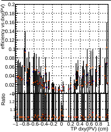
Efficiency vs Dxy(PV) Legend: DQM_mkFit5_QCDHighPt_base DQM_mkFit6_QCDHighPt_retrainOldFiles125_v2_prelimWPM_epoch4 DQM_mkFit5_QCDHighPt_base DQM_mkFit6_QCDHighPt_retrainOldFiles125_v2_prelimWPM_epoch4
