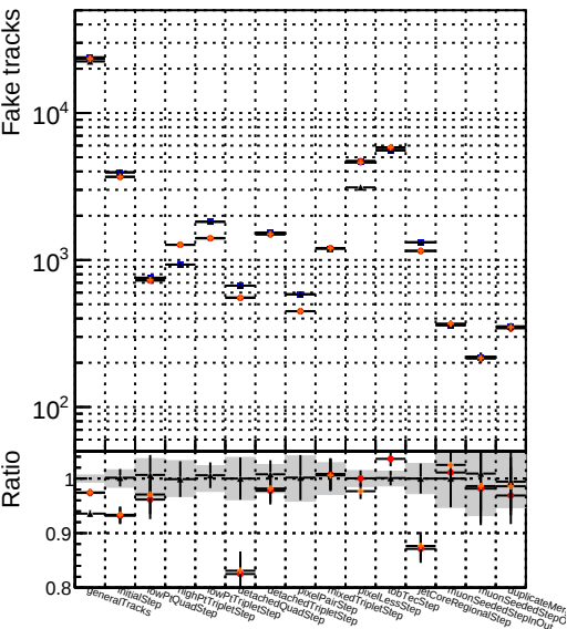
Number Model 1 DQM_mkFit6_QCDHighPt_base 2 DQM_mkFit6_QCDHighPt_retrainOldFiles125_v2_prelimWPM_epoch4
