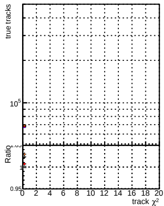
N of reco track vs. \chi^2 for different datasets and WPM versions
