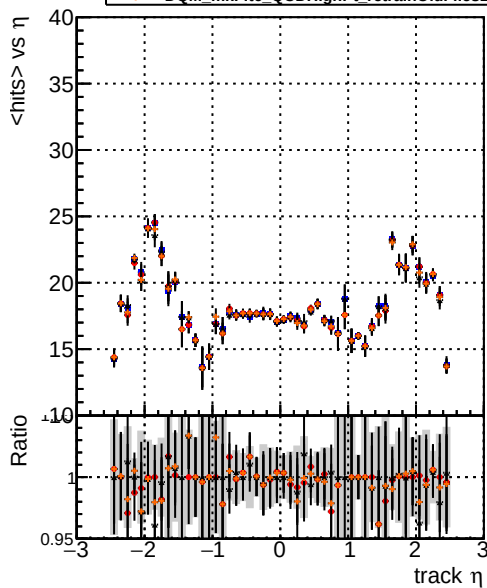
mean hits vs \eta — DQM_mkFit5_QCDHighPt_base — DQM_mkFit5_QCDHighPt_retrainOldFiles125_v2_prelimWPM_epoch4 — DQM_mkFit6_QCDHighPt_base — DQM_mkFit6_QCDHighPt_retrainOldFiles125_v2_prelimWPM_epoch4
