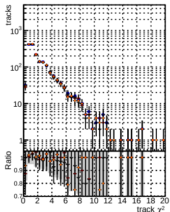
N of reco track vs. \chi^2 for BOM mkt15 OCDF14161 base inOldFiles125 v2_prelimWPM_epoch4
