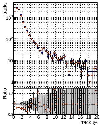
N of reco track vs. \chi^2 for BQM, mKF15, OCB, and HLT base. Legend: BQM (blue), mKF15 (orange), OCB (grey), HLT base (black). Data is shown for inOldFiles125 v2_prelimWPM_epoch4 and retainOldFiles125 v2_prelimWPM_epoch4.
