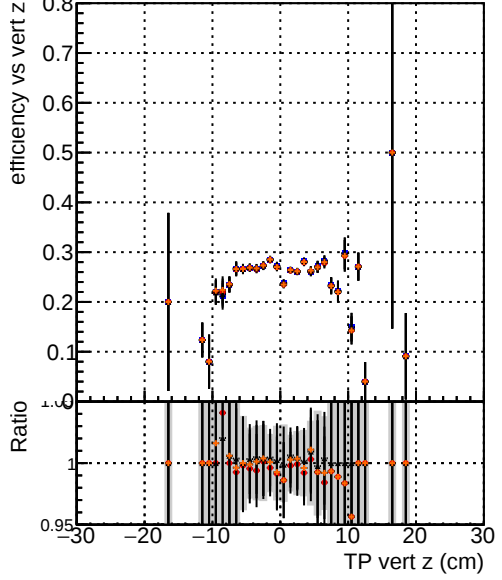
Efficiency vs TP vert z —●— DQM_mkFit5_QCDHighPt_base —●— DQM_mkFit5_QCDHighPt_retrainOldFiles125_v2_prelimWPM_epoch4 —▲— DQM_mkFit6_QCDHighPt_base —▲— DQM_mkFit6_QCDHighPt_retrainOldFiles125_v2_prelimWPM_epoch4
