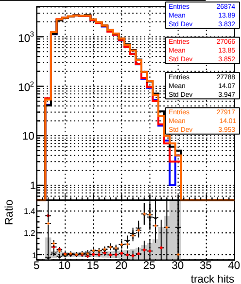
Legend: DOM_mkFit5_QCDHighPt_base DOM_mkFit5_QCDHighPt_retrainOldFiles125_v2_prelimWPM_epoch4 DOM_mkFit6_QCDHighPt_base DOM_mkFit6_QCDHighPt_retrainOldFiles125_v2_prelimWPM_epoch4 mean hits
