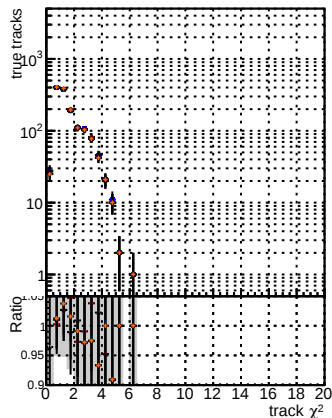
N of reco track vs. \chi^2 for BQM mkt EKF OCB highPt base retainOldFiles125 v2_prelimWPM_epoch4
