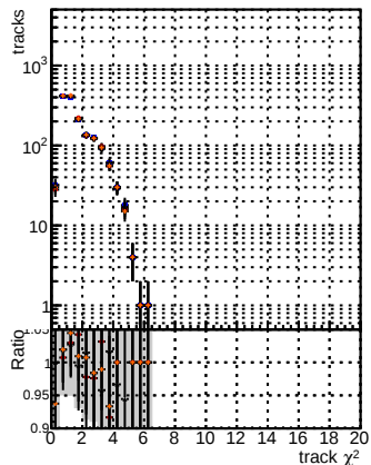
N of reco track vs. \chi^2 for BQM mkt EKF OCB highPt base retainOldFiles125 v2_prelimWPM_epoch4
