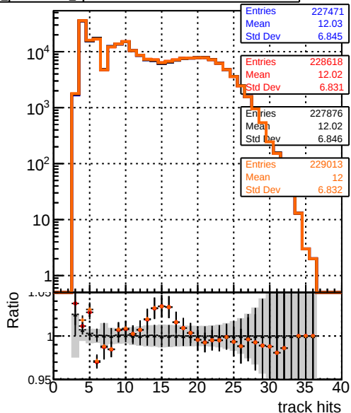
mean hits DOM_mkFit5_QCDHighPt_base DOM_mkFit5_QCDHighPt_retrainOldFiles125_v2_prelimWPM_epoch4 DOM_mkFit6_QCDHighPt_base DOM_mkFit6_QCDHighPt_retrainOldFiles125_v2_prelimWPM_epoch4
