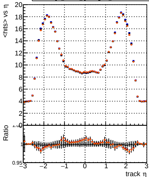
mean hits DOM_mkFit5_QCDHighPt_base DOM_mkFit5_QCDHighPt_retrainOldFiles125_v2_prelimWPM_epoch4 DOM_mkFit6_QCDHighPt_base DOM_mkFit6_QCDHighPt_retrainOldFiles125_v2_prelimWPM_epoch4
