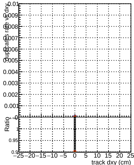
DOM mkt5 OGDHighPt base retainOldFiles125_v2_prelimWPM_epoch4 DOM mkt5 OGDHighPt base retainOldFiles125_v2_prelimWPM_epoch4
