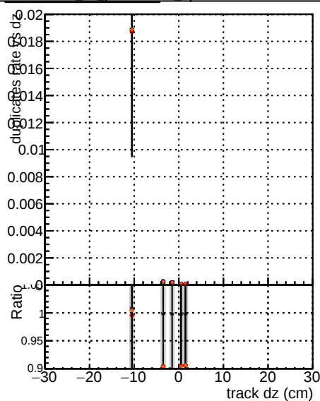
DOM mkt5 OGDHighPt base retainOldFiles125_v2_prelimWPM_epoch4 DOM mkt5 OGDHighPt base retainOldFiles125_v2_prelimWPM_epoch4
