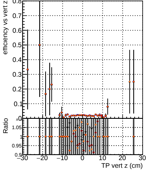
Efficiency vs vert z —●— DQM_mkFit5_QCDHighPt_base —●— DQM_mkFit5_QCDHighPt_retrainOldFiles125_v2_prelimWPM_epoch4 —●— DQM_mkFit6_QCDHighPt_base —●— DQM_mkFit6_QCDHighPt_retrainOldFiles125_v2_prelimWPM_epoch4
