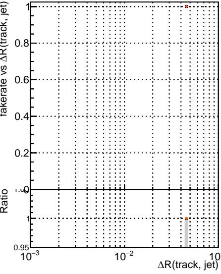
Fake rate vs \Delta R(\text{track, jet}) base trainOldFiles125_v2_prelimWPM_epoch4 DQM mkFI15 QCDHighPT base DQM mkFI16 QCDHighPT trainOldFiles125_v2_prelimWPM_epoch4
