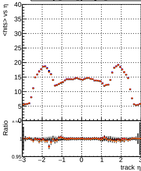
mean hits — DQM_mkFit5_QCDHighPt_base — DQM_mkFit5_QCDHighPt_retrainOldFiles125_v2_prelimWPM_epoch4 — DQM_mkFit6_QCDHighPt_base — DQM_mkFit6_QCDHighPt_retrainOldFiles125_v2_prelimWPM_epoch4
