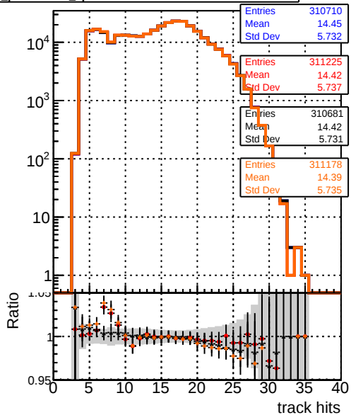
mean hits — DQM_mkFit5_QCDHighPt_base — DQM_mkFit5_QCDHighPt_retrainOldFiles125_v2_prelimWPM_epoch4 — DQM_mkFit6_QCDHighPt_base — DQM_mkFit6_QCDHighPt_retrainOldFiles125_v2_prelimWPM_epoch4
