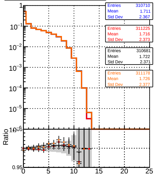
mean hits — DQM_mkFit5_QCDHighPt_base — DQM_mkFit5_QCDHighPt_retrainOldFiles125_v2_prelimWPM_epoch4 — DQM_mkFit6_QCDHighPt_base — DQM_mkFit6_QCDHighPt_retrainOldFiles125_v2_prelimWPM_epoch4
