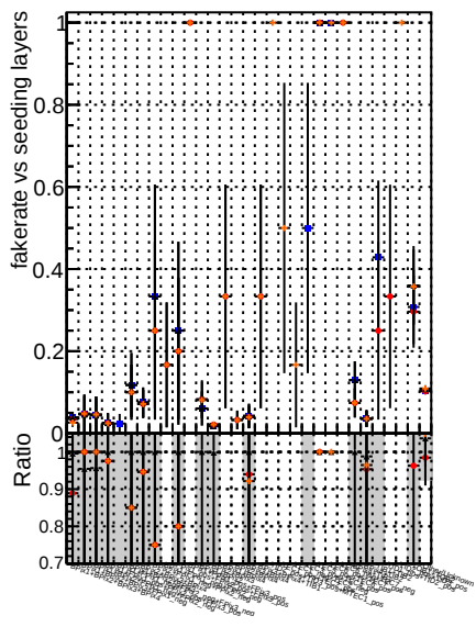
Fake rate vs. BSM mkl i5 GCD high PL retainOldFiles125_v2_prelimWPM_epoch4 retainOldFiles125_v2_prelimWPM_epoch4
