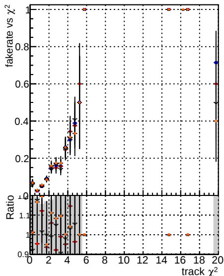
Fake rate vs. BSM mkl i5 GCD high PL retainOldFiles125_v2_prelimWPM_epoch4 retainOldFiles125_v2_prelimWPM_epoch4
