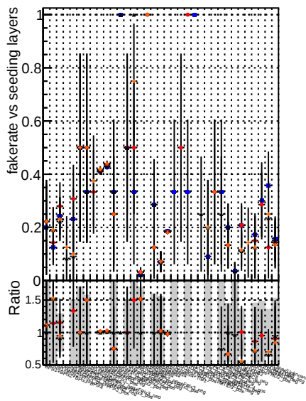
Fake rate vs. DGM mkFit5 OGDHighBL base DGM mkFit6 OGDHighBL v2 retainOldFiles125 v2_prelimWPM_epoch4 retainOldFiles125 v2_prelimWPM_epoch4
