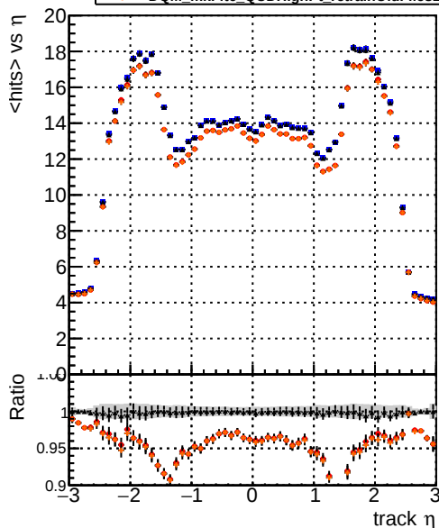
mean hits vs \eta Legend: — DQM_mkFit5_QCDHighPt_base — DQM_mkFit5_QCDHighPt_retrainOldFiles125_v2_prelimWPM_epoch4 — DQM_mkFit6_QCDHighPt_base — DQM_mkFit6_QCDHighPt_retrainOldFiles125_v2_prelimWPM_epoch4
