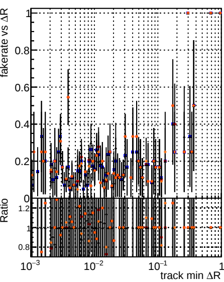
Fake rate vs \Delta R(\text{track, jet}) for various models and datasets. The legend includes: DOM, mkt, mkt15, mkt16, OCB, HighPt, base, retrainOldFiles125_v2_prelimWPM_epoch4, and retrainOldFiles125_v2_prelimWPM_epoch4.
