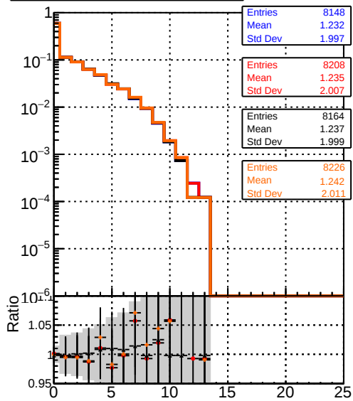
— DQM_mkFit5_QCDHighPt_base — DQM_mkFit5_QCDHighPt_retrainOldFiles125_v2_prelimWPM_epoch4 — DQM_mkFit6_QCDHighPt_base — DQM_mkFit6_QCDHighPt_retrainOldFiles125_v2_prelimWPM_epoch4
