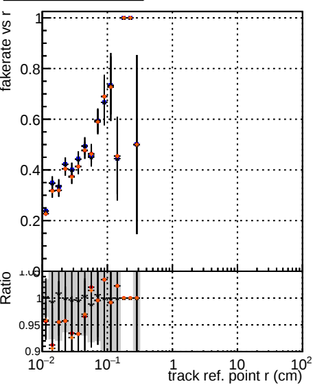
DOM mktF15 OCBHighPt base DOM mktF16 OCBHighPt base DOM mktF16 OCBHighPt base retrainOldFiles125_v2_prelimWPM_epoch4 retrainOldFiles125_v2_prelimWPM_epoch4
