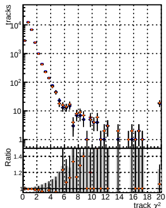
N of reco track vs. \chi^2 for BSM, mkt, E5, OCDF, and HighPt base. Legend: BSM mkt E5 OCDF HighPt base. Data source: OldFiles125 v2_prelimWPM_epoch4.
