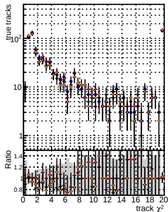
N of reco track vs. \chi^2 for BSM, mkt15, OCB, highPt base, inOldFiles125_v2_prelimWPM_epoch4, retainOldFiles125_v2_prelimWPM_epoch4
