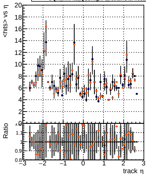
mean hits — DQM_mkFit5_QCDHighPt_base — DQM_mkFit5_QCDHighPt_retrainOldFiles125_v2_prelimWPM_epoch4 — DQM_mkFit6_QCDHighPt_base — DQM_mkFit6_QCDHighPt_retrainOldFiles125_v2_prelimWPM_epoch4
