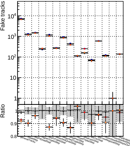
Number Model 1 DQM mkFit6 QCDHighPt_base 2 DQM mkFit6 QCDHighPt_retrainOldFiles125_v2_prelimWPM_epoch4
