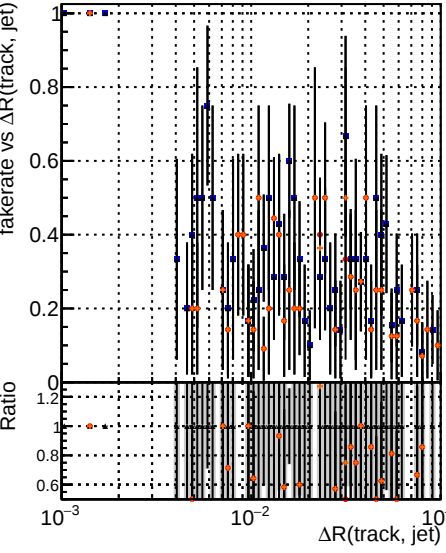
Fake rate vs \Delta R(\text{track, jet}) Legend: DOM mkr15 mkr16 OGD highpt base retrainOldFiles125_v2_prelimWPM_epoch4 retrainOldFiles125_v2_prelimWPM_epoch4
