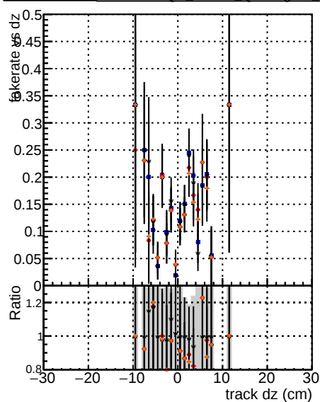
Fake rate vs dz DOM mkFit5 OGDHighPT base trainOldFiles125_v2_prelimWPM_epoch4 DOM mkFit6 OGDHighPT base trainOldFiles125_v2_prelimWPM_epoch4
