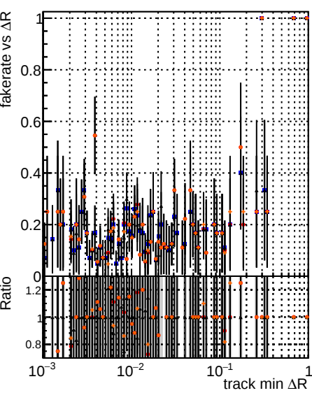
Fake rate vs \Delta R(\text{track, jet}) base trainOldFiles125_v2_prelimWPM_epoch4 trainOldFiles125_v2_prelimWPM_epoch4
