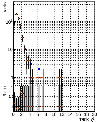
N of reco track vs. \chi^2 for BQM, mkt, OCB, and HBT bases in OldFiles125 v2_prelimWPM_epoch4
