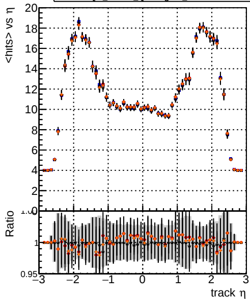
mean hits vs \eta Legend: - DQM_mkFit5_QCDHighPt_base (blue line) - DQM_mkFit5_QCDHighPt_retrainOldFiles125_v2_prelimWPM_epoch4 (red line with dots) - DQM_mkFit6_QCDHighPt_base (black line with dots) - DQM_mkFit6_QCDHighPt_retrainOldFiles125_v2_prelimWPM_epoch4 (orange line with dots)
