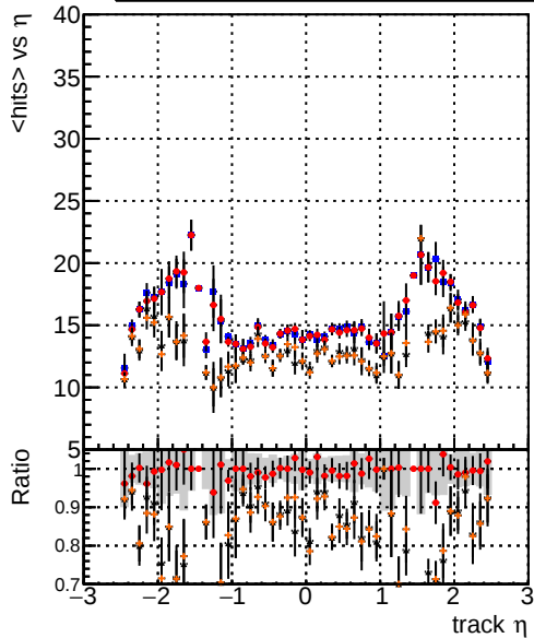
mean hit — DQM_mkFit5_QCDHighPt_base — DQM_mkFit5_QCDHighPt_retrainOldFiles125_v2_prelimWPM_epoch4 — DQM_mkFit6_QCDHighPt_base — DQM_mkFit6_QCDHighPt_retrainOldFiles125_v2_prelimWPM_epoch4
