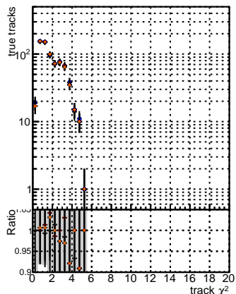
N of reco track vs. \chi^2 for BGM, mEFT, F15, OCB, HighPt, PL base, retainOldFiles125_v2_prelimWPM_epoch4
