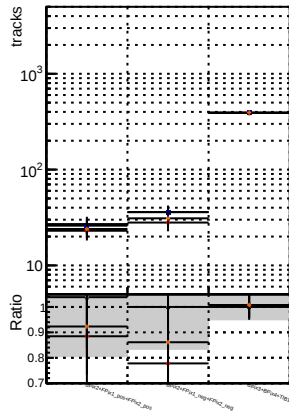
N of reco track vs. \chi^2 for BQM, mkt, E5, OCB, and HARP. Data from OldFiles125_v2_prelimWPM_epoch4 and retainOldFiles125_v2_prelimWPM_epoch4.
