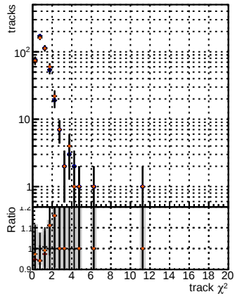
N of reco track vs. \chi^2 for BQM, mkt, E5, OCB, and HARP. Data from OldFiles125_v2_prelimWPM_epoch4 and retainOldFiles125_v2_prelimWPM_epoch4.
