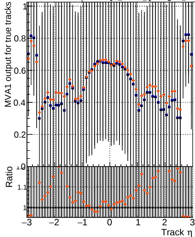
MVA1 of associated tracks (recoToSim) vs. track \eta Legend: DQM_mkFit5_QCDHighPt_base (blue squares) DQM_mkFit5_QCDHighPt_retrainOldFiles125_v2_prelimWPM_epoch4 (red circles) DQM_mkFit6_QCDHighPt_base (black triangles) DQM_mkFit6_QCDHighPt_retrainOldFiles125_v2_prelimWPM_epoch4 (orange diamonds)
