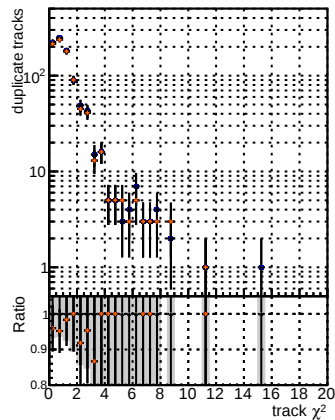
N of associated (recoToSim) lepton tracks vs normalized \chi^2
