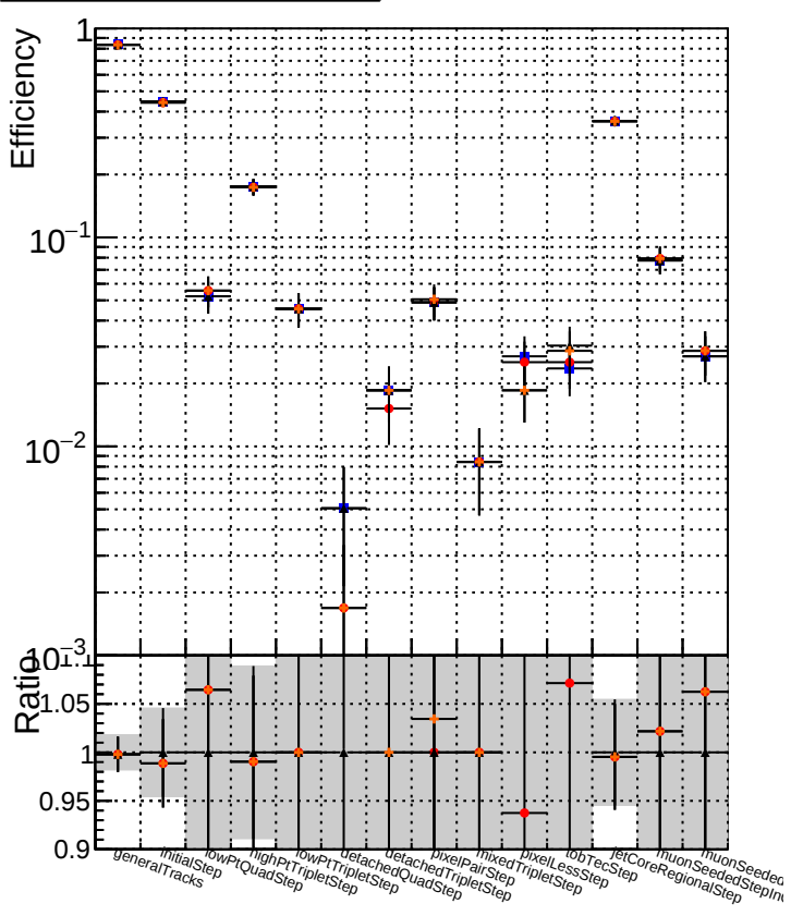
Legend: DQM_mkFit5_QCDHighPt_base DQM_mkFit5_QCDHighPt_retrainOldFiles125_v2_prelimWPM_epoch4 DQM_mkFit6_QCDHighPt_base DQM_mkFit6_QCDHighPt_retrainOldFiles125_v2_prelimWPM_epoch4
