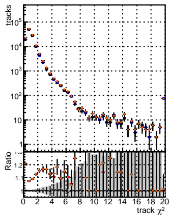
N of reco track vs. \chi^2 for BGM, mkt16, OCB, HighPt, beta, inOldFiles125_v2_prelimWPM_epoch4, mkt16, OCB, HighPt, beta, inOldFiles125_v2_prelimWPM_epoch4, mkt16, OCB, HighPt, beta, inOldFiles125_v2_prelimWPM_epoch4
