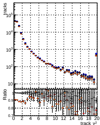
N of reco track vs. \chi^2 for BQM, mkt15, OCB, HighET, base, retainOldFiles125 v2, prelimWPM_epoch4
