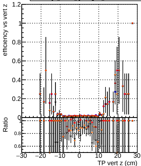
Efficiency DOM mkFit5 QCDHighPt retrainOldFiles125 v2 prelimWPM epoch4 DOM mkFit6 QCDHighPt base DOM mkFit6 QCDHighPt retrainOldFiles125 v2 prelimWPM epoch4
